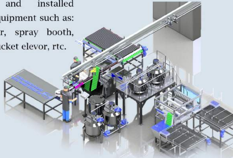
Inline Filling Machine
